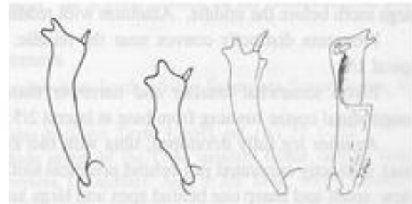
a b c d Fig. 6 Anterior tibia of Colophon spp. a, C. eastmanii nagaii ssp. nov., male ; b, do., female ; c, C. e. eastmanii , male ; d, do. (in semi-ventral view) (c-d, after S. Endrody-Younga, 1988).
